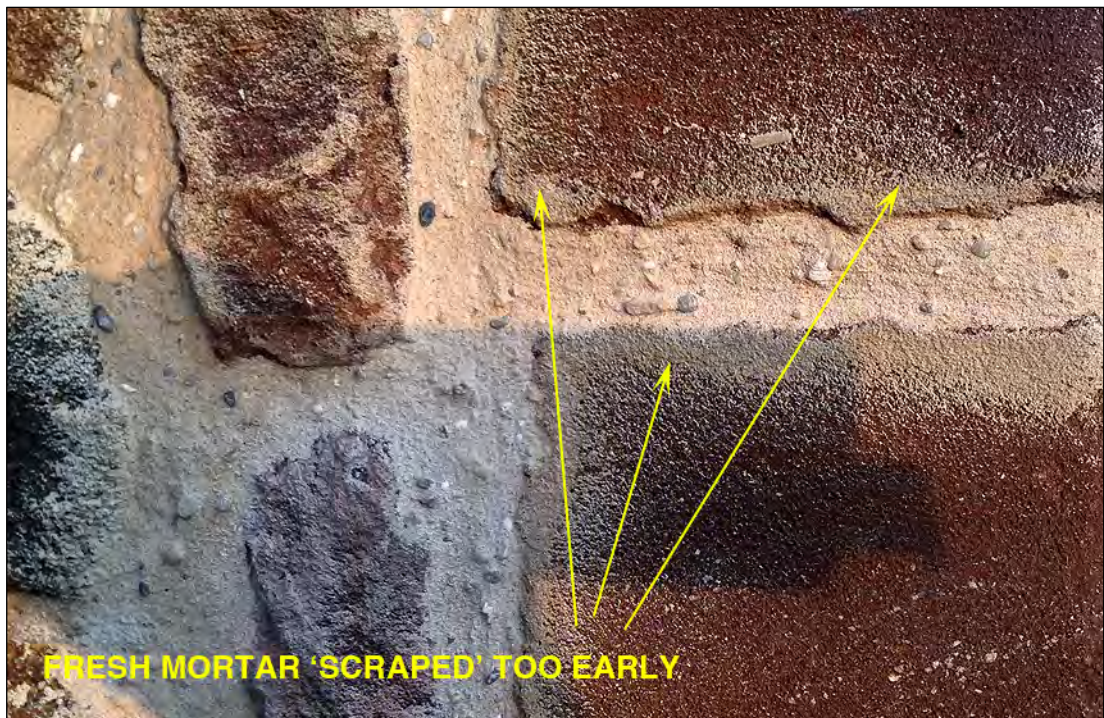
C.06: PERMANENT DISCOLOURATION OF STONework DUE TO ATTEMPT TO REMOVE SURPLUS MORTAR WHILE PLACING (I.E. WHEN FRESH)
