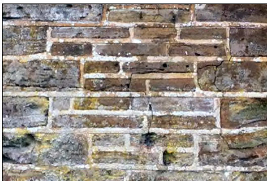
C.15: SQUARED BROUGHT TO COURSES
