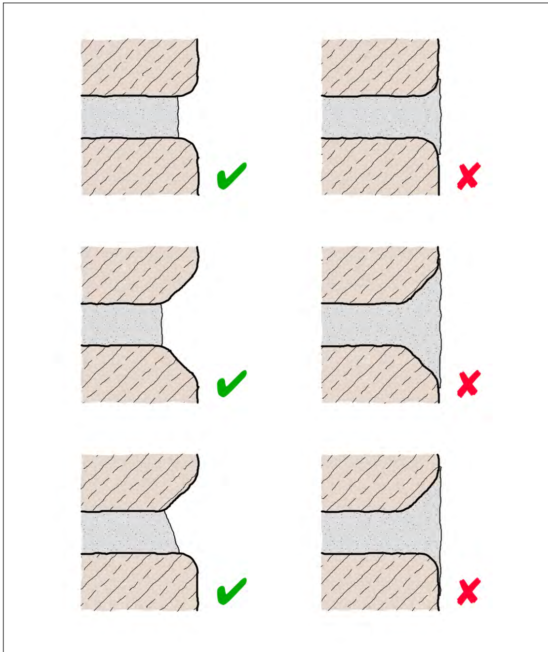
C.07: CORRECT & INCORRECT TREATMENT OF POINTED JOINTS
